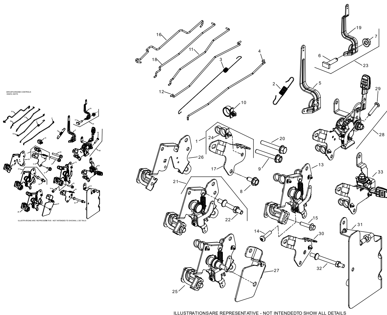
GROUP 9-ENGINE CONTROLS HD675, HD775
